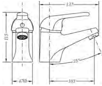
Ref.: 60130 06 45 66 Monomando de lavabo Single lever wash-basin mixer
