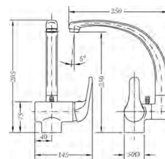
Ref.: 61900 06 45 66 Monomando de fregadera abatible Single lever folding sink mixer
