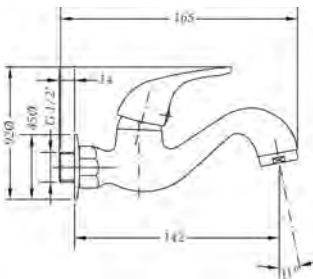
Ref.: 1006 04 Grifo lavabo mural 1 agua cartucho 25 1 water wall wash basin cartridge 25
