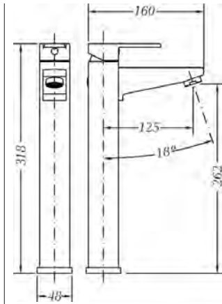
Ref.: 63136 26 45 66 Monomando de lavabo alto High single lever wash-basin mixer
