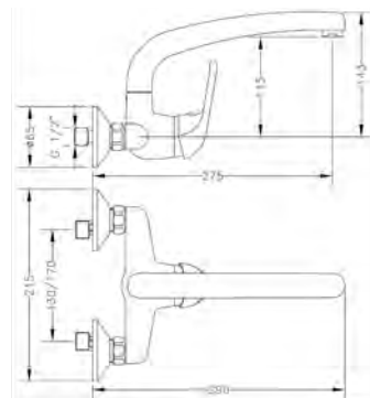
Ref.: 61192 06 45 66 Monomando de fregadera mural 15 cm Single-lever wall sink mixer 15 cm
