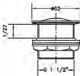
Ref.: 100208 45 Válvula click 1 1/4" bañera 1 1/4" bath click valve
