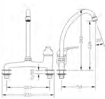
Ref.: 60198 05 45 66 Monomando mesada 8" 8" wide spread single lever sink mixer
