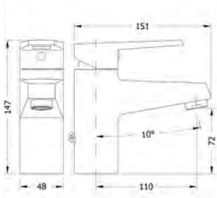
Ref.: 64130 14 45 66 Monomando de lavabo Single lever wash-basin mixer
