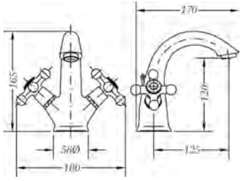
Ref.: 68506 09 45 66 Monobloc de lavabo cromo Wash basin mixer chromed
