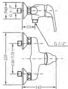
Ref.: 60110 06 45 66 Monomando de ducha con kit Single lever shower mixer with kit
