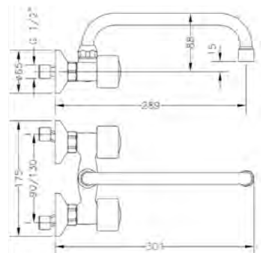
Ref.: 68196 11 45 66 Grupo mural fregadera 11 cm caño tubo alto 24cm Wall sink mixer 11 cm with high tube spout 24cm
