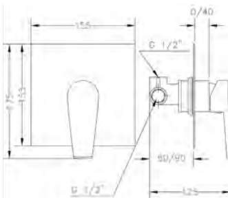
Ref.: 64115 16 45 66 Monomando de ducha empotrado Built-in single lever shower
