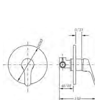
Ref.: 61115 22 45 66 Monomando de ducha empotrado Built-in single lever shower
