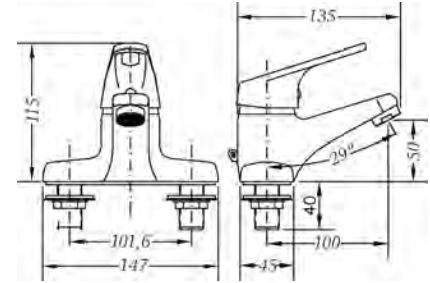
Ref.: 60188 22 45 66 Monomando de lavabo centerset 4" Single lever wash-basin mixer 4" centerset
