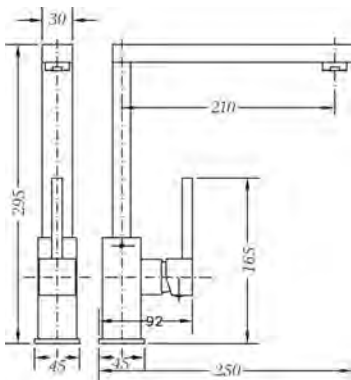
Ref.: FRK63400 Monomando de fregadera cartucho 25 Single lever sink mixer cartridge 25
