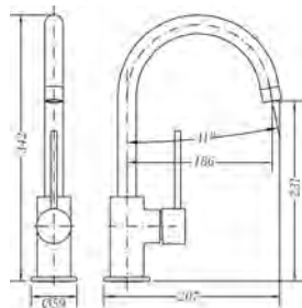
Ref.: FRT65402 Monomando de fregadera cartucho 35 Single lever sink mixer cartridge 35
