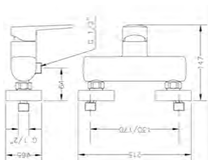
Ref.: 64110 04 45 66 Monomando de ducha con kit Single lever shower mixer with kit
