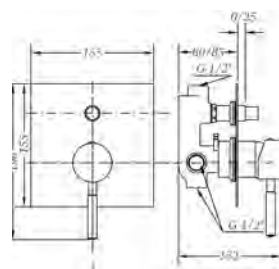
Ref.: 65116 18 45 66 Monomando de baño empotrado con inversor Built-in single lever bath with diverter
