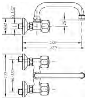
Ref.: 68195 11 45 66 Grupo mural fregadera 11 cm caño tubo alto 18cm Wall sink mixer 11 cm with high tube spout 18cm
