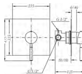
Ref.: 65115 18 45 66 Monomando de ducha empotrado Built-in single lever shower
