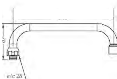
Ref.: 68902 45 Caño alto tubo 24 cm High tube spout 24 cm
