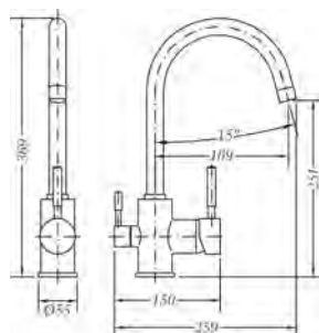
Ref.: 65702 18 45 66 Monomando de fregadera Osmosis cartucho 35 Single lever sink Osmosis mixer 35 cartridge
