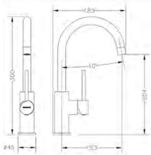
Ref.: 65138 18 45 66 Monomando de lavabo Single lever wash-basin tap
