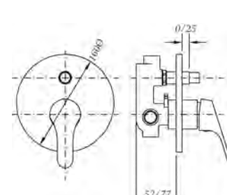
Ref.: 61116 22 45 66 Monomando de baño empotrado con inversor Built-in single lever bath with diverter
