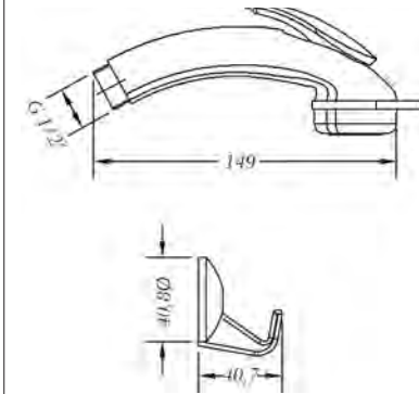
Ref.: 100696 45 Kit soporte y ducha sanitaria holder and sanitary shower kit
