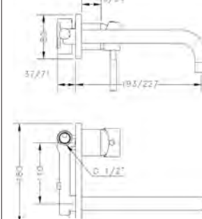
Ref.: 65132 18 45 66 Monomando de lavabo empotrado caño 22cm Built-in wash-basin mixer 22 cm spout
