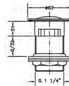
Ref.: 100206 45 Válvula click 1 1/4" con rebosadero 1 1/4" click valve with overflow
