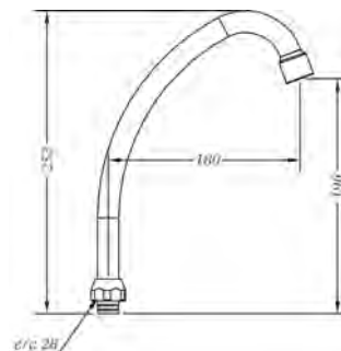
Ref.: 68903 45 Caño tubo vertical Swan neck spout
