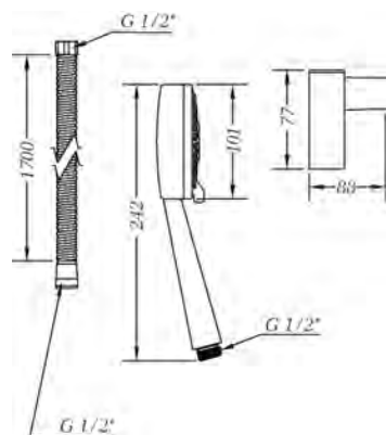
Ref.: 100698 45 Kit de ducha Kenjo, flexo, soporte y ducha 3 jets (caja) Kenjo shower set, flexible hose, holder and 3 jets handshower (box)
