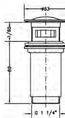
Ref.: 100209 45 Válvula click 1 1/4" con/sin rebosadero 1 1/4" click valve with/out overflow
