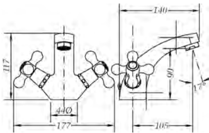
Ref.: 68505 09 45 66 Monobloc de lavabo Wash basin mixer
