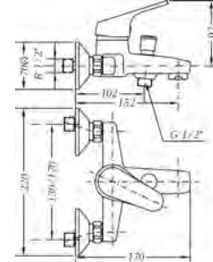
Ref.: 60100 22 45 66 Monomando de baño con kit Single lever bath mixer with kit
