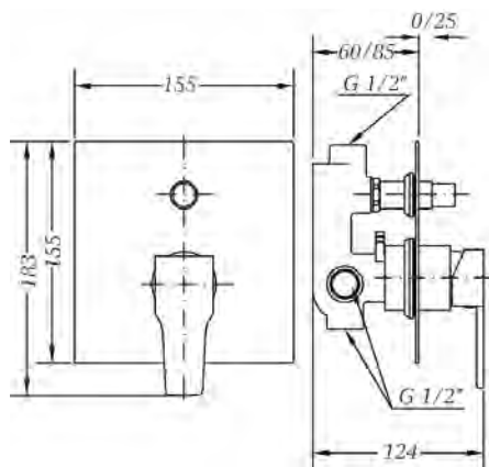
Ref.: 63116 26 45 66 Monomando de baño empotrado con inversor Built-in single lever bath with diverter
