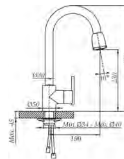
Ref.: FRV61205 Monomando de fregadera ducha extraíble Single lever sink mixer with pull-out spray
