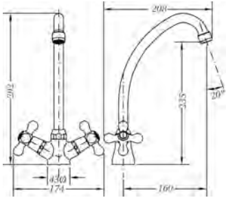
Ref.: 68540 09 45 66 Monobloc fregadera caño tubo Sink mixer goose neck spout
