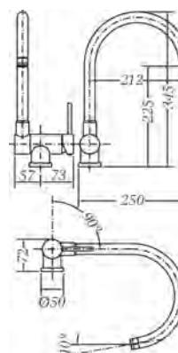
Ref.: 65900 18 45 66 Monomando de fregadera abatible cartucho 35 Single lever folding sink mixer 35 cartridge
