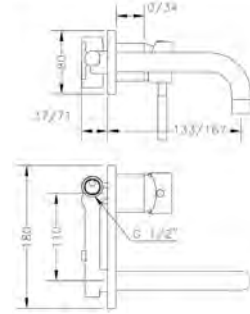
Ref.: 65131 18 45 66 Monomando de lavabo empotrado caño 16cm Built-in wash-basin mixer 16 cm spout
