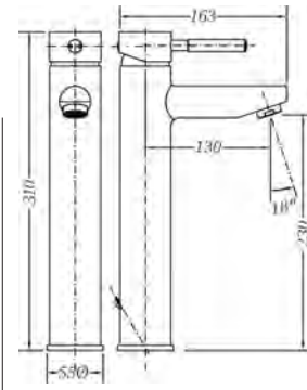
Ref.: 65136 18 45 66 Monomando de lavabo alto High single lever wash-basin mixer
