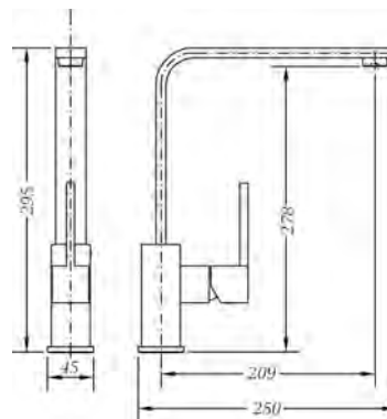
Ref.: FRK63401 Monomando de fregadera cartucho 25 Single lever sink mixer cartridge 25
