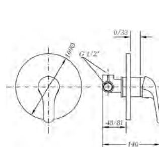
Ref.: 61115 06 45 66 Monomando de ducha empotrado Built-in single lever shower
