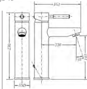
Ref.: 65134 18 45 66 Monomando de lavabo medio alto Medium high single lever wash-basin mixer
