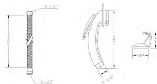
Ref.: 100141 Flexo 1,20m. inoxidable Stainless steel flexible hose 1,20 m. Box: 1 | Carton: 50 | Pallet: 900
