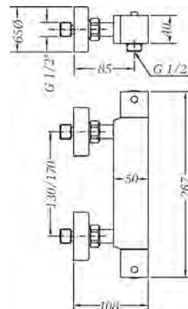
Ref.: 67110 26 45 67 Termostática ducha sin kit Thermostatic shower without kit
