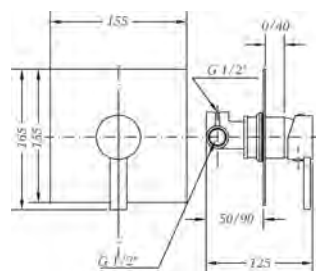
Ref.: 65115 29 45 66 Monomando de ducha empotrado Built-in single lever shower
