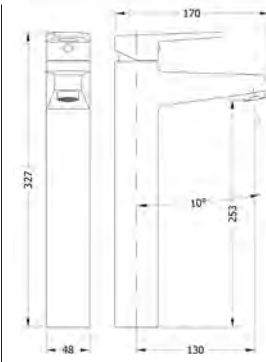
Ref.: 64136 14 45 66 Monomando de lavabo alto High single lever wash-basin mixer
