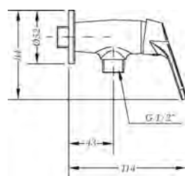
Ref.: 60001 22 45 67 Grifo bide mural 1 agua cartucho 25 1 water wall bidet 25 cartridge
