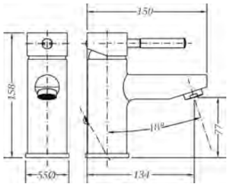
Ref.: 65135 18 45 66 Monomando de lavabo Single lever wash-basin tap
