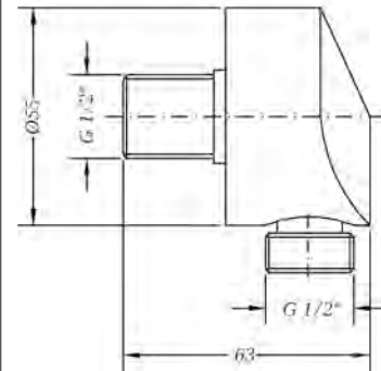
Ref.: 1680 04 Toma ducha mural redonda Round wall flexible connector
