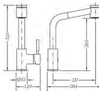
Ref.: 65205 18 45 66 Monomando de fregadera ducha extraíble Single lever sink mixer with pull-out spray
