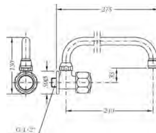
Ref.: 68093 11 45 66 Grifo mural fregadera caño tubo alto 24cm Wall sink tap with tube spout 24cm
