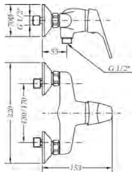
Ref.: 60110 22 45 66 Monomando de ducha con kit Single lever shower mixer with kit
