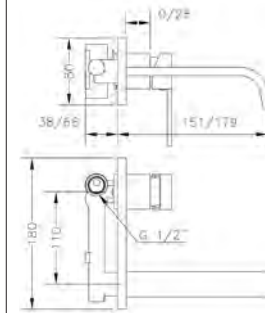
Ref.: 63131 26 45 66 Monomando de lavabo empotrado caño 16cm Built-in wash-basin mixer 16 cm spout
