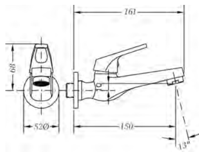
Ref.: 1003 04 Grifo lavabo mural 1 agua cartucho 25 1 water wall wash basin 25 cartridge
