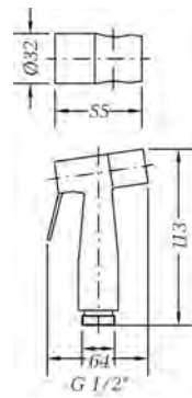
Ref.: 100694 60 Kit ducha sanitaria. Inox Inox sanitary shower kit
