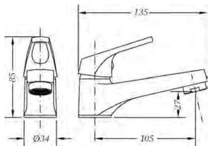
Ref.: 1002 04 Grifo lavabo 1 agua cartucho 25 1 water wash basin 25 cartridge
