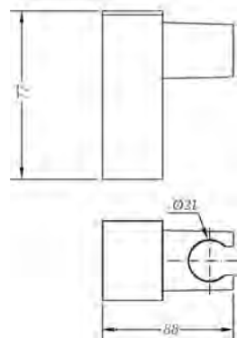
Ref.: 100149 45 Soporte ducha Kenjo Kenjo shower holder
