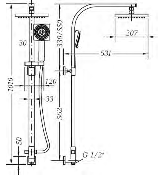
Ref.: 1746 45 Set columna extensible con ducha, soporte y flexo Extensible column set with shower, holder and flexible hose
