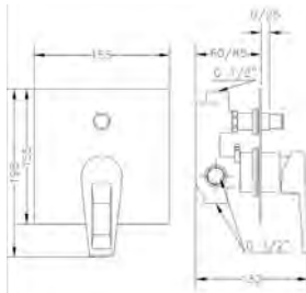
Ref.: 64116 14 45 66 Monomando de baño empotrado con invector Built-in single lever bath with diverter
