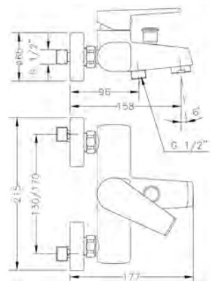
Ref.: 64100 04 45 66 Monomando de baño con kit Single lever bath mixer with kit
