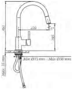
Ref.: FRV61206 Monomando de fregadera caño extraíble Single-lever sink mixer with pull-out spout
