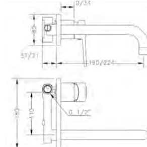
Ref.: 64132 14 45 66 Monomando de lavabo empotrado caño 22 cm Built-in wash-basin mixer 22 cm spout
