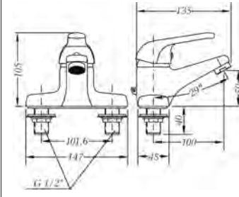
Ref.: 60188 06 45 66 Monomando de lavabo centerset 4" Single lever wash-basin mixer 4" centerset
