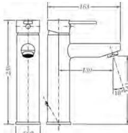
Ref.: 65134 29 45 66 Monomando de lavabo medio alto Medium high single lever wash-basin mixer
