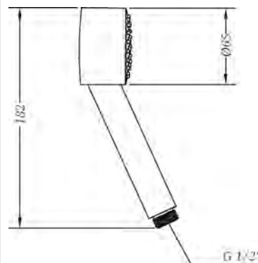
Ref.: 100197 45 00 Mango de ducha C1 jet (bolsa) C1 jet handshower (bag)
