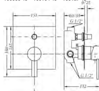
Ref.: 65116 29 45 66 Monomando de baño empotrado con inversor Built-in single lever bath with diverter
