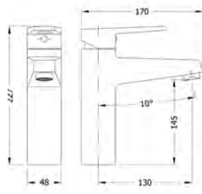
Ref.: 64134 14 45 66 Monomando de lavabo medio alto Medium high single lever wash-basin mixer
