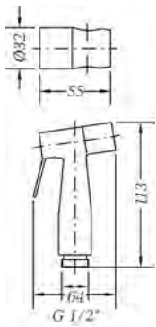
Ref.: 100694 45 Kit ducha sanitaria Sanitary shower kit
