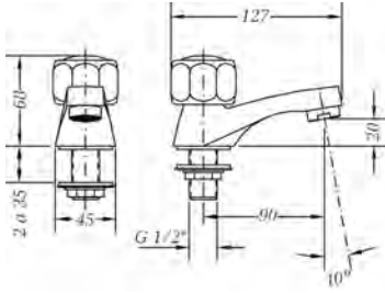
Ref.: 68180 11 45 66 Grifo de lavabo Wash basin tap
