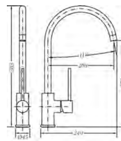
Ref.: FRT65401 Monomando de fregadera cartucho 25 Single lever sink mixer cartridge 25
