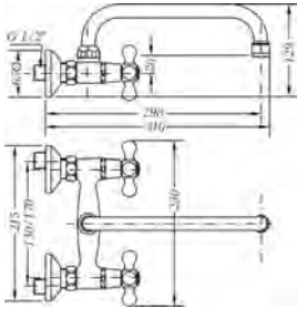
Ref.: 68555 09 45 66 Grupo mural fregadera 15 cm caño tubo alto 24cm Wall mounted sink mixer 15 cm with high tube spout 24cm
