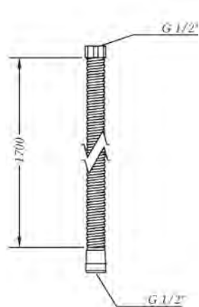
Ref.: 100135 60 00 Flexo 1,70 m inoxidable Stainless steel flexible hose 1,70 m
