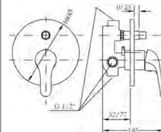
Ref.: 61116 06 45 66 Monomando de baño empotrado con inversor Built-in single lever bath with diverter
