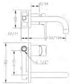
Ref.: 64131 14 45 66 Monomando de lavabo empotrado caño 16 cm Built-in wash-basin mixer 16 cm spout
