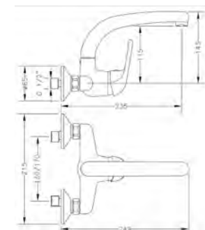
Ref.: 61190 06 45 66 Monomando de fregadera mural 15 cm caño corto Wall single lever sink mixer 15cm short spout
