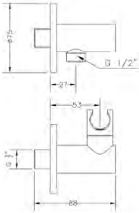
Ref.: 1633 04 Soporte ducha con toma cilindrico Round shower holder with flexible connector
