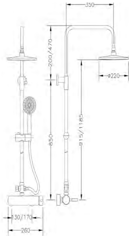
Ref.: CM65110 18 Columna monomando extensible con kit Single lever extensible column with kit
