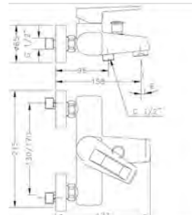
Ref.: 64100 14 45 66 Monomando de baño con kit Single lever bath mixer with kit
