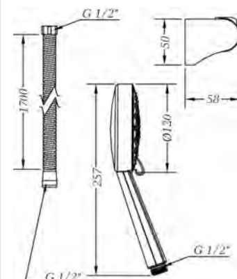
Ref.: 100699 45 Kit de ducha Tau, flexo, soporte y ducha 5 jets (caja) Tau shower set, flexible hose, holder and 5 jets handshower (box)
