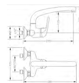
Ref.: 61195 06 45 66 Monomando de fregadera mural 11 cm Wall single lever sink mixer 11 cm
