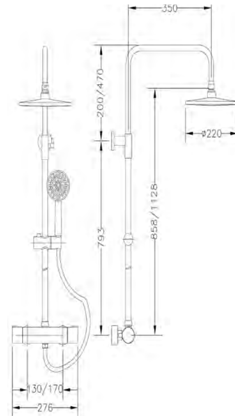
Ref.: CT67110 18 Columna termostática extensible con kit Thermostatic extensible column with kit
