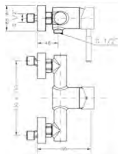
Ref.: 65110 18 45 66 Monomando de ducha con kit Single lever shower mixer with kit
