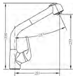
Ref.: 61206 06 45 66 Monomando de fregadera ducha extraíble Single-lever sink mixer with pull-out spray
