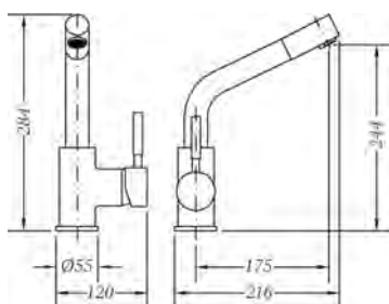
Ref.: 65206 18 45 66 Monomando de fregadera caño extraíble Single lever sink mixer with pull-out spout
