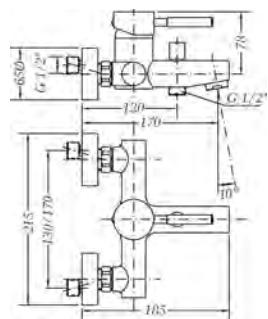
Ref.: 65100 18 45 66 Monomando de baño con kit Single lever bath mixer with kit
