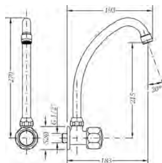
Ref.: 68083 11 45 66 Grifo fregadera mural caño tubo vertical Wall sink tap with swan neck spout
