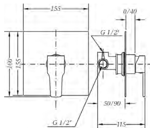
Ref.: 63115 26 45 66 Monomando de ducha empotrado Built-in single lever shower
