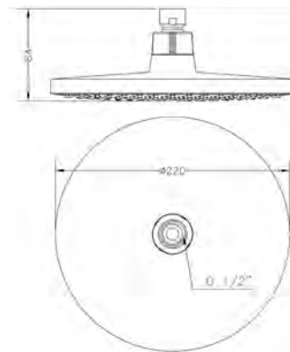
Ref.: R65112 18 Rociador redondo 22 cm Round shower head Ø 22 cm
