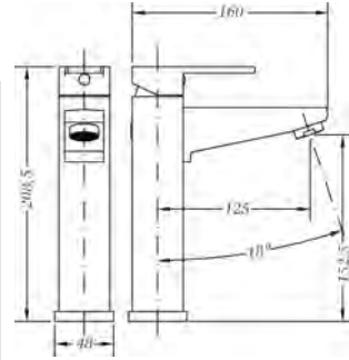
Ref.: 63134 26 45 66 Monomando de lavabo medio alto Medium high single lever wash-basin mixer
