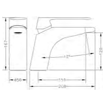
Ref.: 62130 08 45 66 Monomando de lavabo Single lever wash-basin mixer
