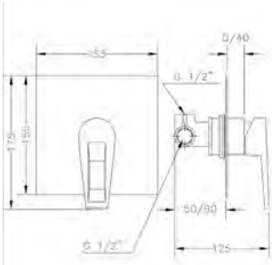
Ref.: 64115 14 45 66 Monomando de ducha empotrado Built-in single lever shower
