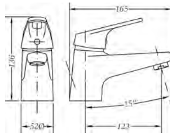
Ref.: 60130 22 45 66 Monomando de lavabo Single lever wash-basin mixer
