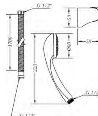
Ref.: 100697 45 Kit de ducha GE2, flexo, soporte y ducha 1 jet (caja) GE2 shower set, flexible hose, holder and 1 jet handshower (box)
