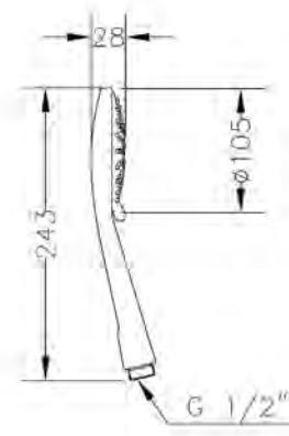
Ref.: DXT3 45 Mango de ducha T3 jets (caja) T3 jets handshower (box)
