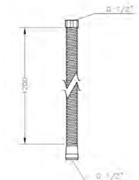
Ref.: 100141 45 Flexo 1,20 m inoxidable Stainless steel flexible hose 1,20 m
