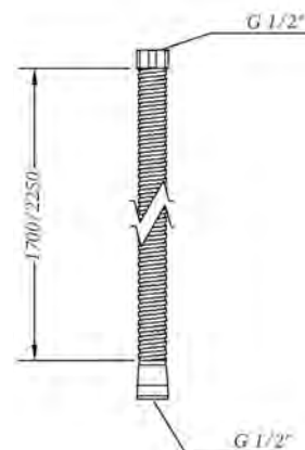
Ref.: 100137 60 00 Flexo extensible 1,70 - 2,25 m inoxidable doble grapaje Extendable stainless steel flexible hose 1,70 to 2,25 m double lock
