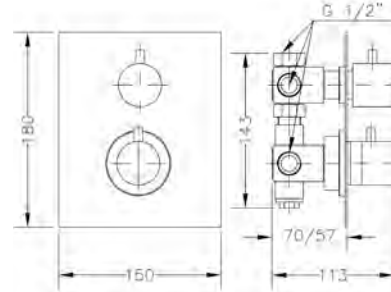
Ref.: 64114 14 45 67 Termostática empotrada 2 salidas Built-in thermostatic 2 outlets
