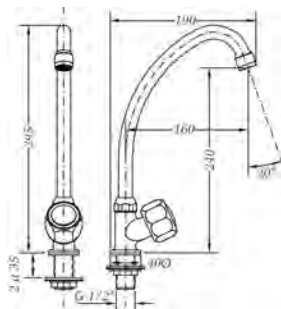
Ref.: 68003 11 45 66 Grifo fregadera caño tubo vertical Sink tap with vertical swan neck spout
