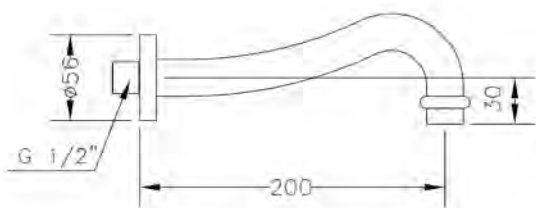
Ref.: 68914 45 Caño mural tubo retro 20 cm Wall mounted retro pipe spout 20 cm
