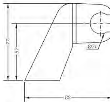
Ref.: 100152 45 Soporte ducha Combi Combi shower holder
