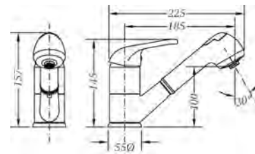
Ref.: 61205 06 45 66 Monomando de fregadera ducha extraíble Single lever sink mixer with pull-out spray
