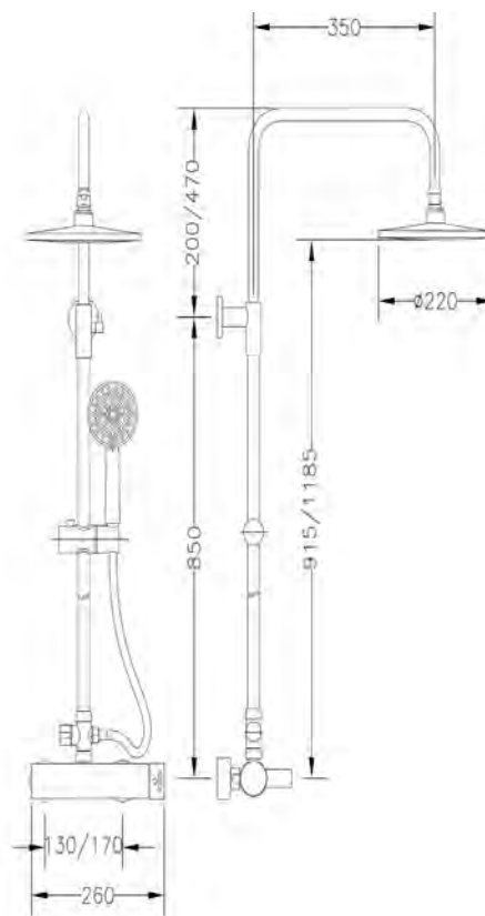
Ref.: CM65110 29 Columna monomando extensible con kit Single lever extensible column with kit
