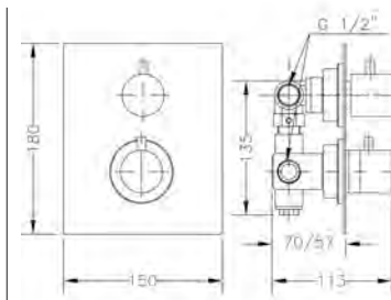
Ref.: 64111 14 45 67 Termostática empotrada 3 salidas Built-in thermostatic 3 outlets
