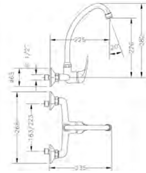
Ref.: 60194 05 45 66 Monomando de fregadera mural 8" Wall single lever 8" sink mixer
