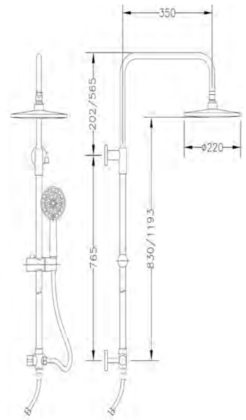
Ref.: 1745 45 Set columna extensible con ducha, soporte y flexo Extensible column set with shower, holder and flexible hose
