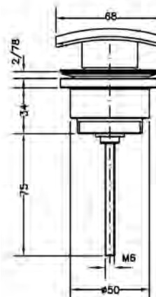
Ref.: 100204 45 Válvula click Kenjo 1 1/4" 1 1/4" Kenjo click valve
