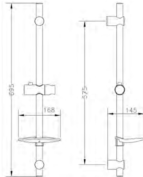
Ref.: 1636 45 Barra ducha TAU (caja) TAU shower bar (box)
