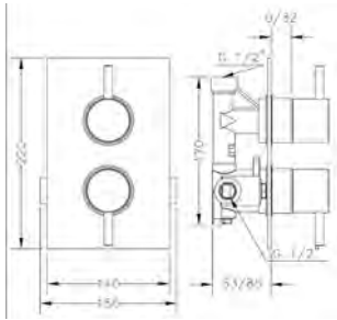
Ref.: 64113 14 45 67 Termostática empotrada 1 salida Built-in thermostatic 1 outlet
