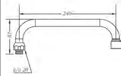
Ref.: 68902 45 Caño alto tubo 24 cm High tube spout 24 cm
