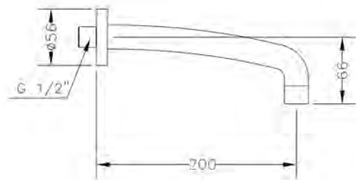
Ref.: 68913 45 Caño mural tubo inclinado 20 cm Wall mounted sloping pipe spout 20 cm
